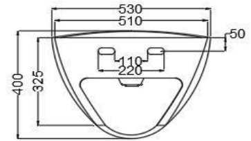
BACK VIEW
