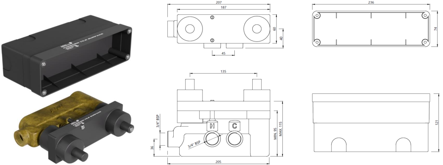
THERMOSTATIC SHOWER MIXER BODY
